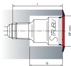
Flush socket
