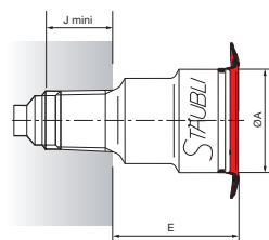
Proud socket
