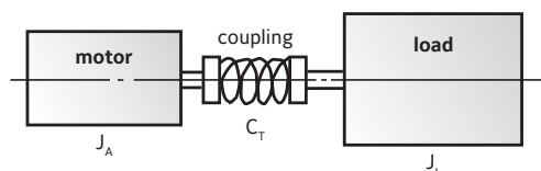
Two Mass System
