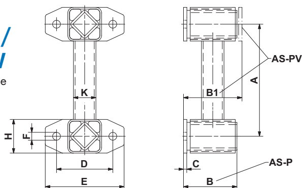
Type AS-PV with inverted flange
