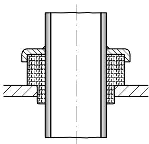
Pipe isolation.
