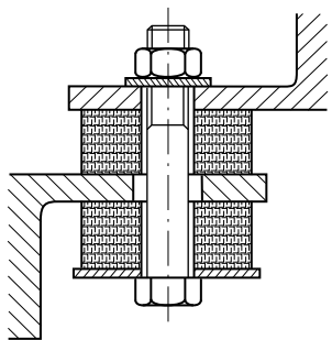
Suspension of gearboxes, motors, fans, pumps, axial load only. A gap is necessary around the fixing screw.
